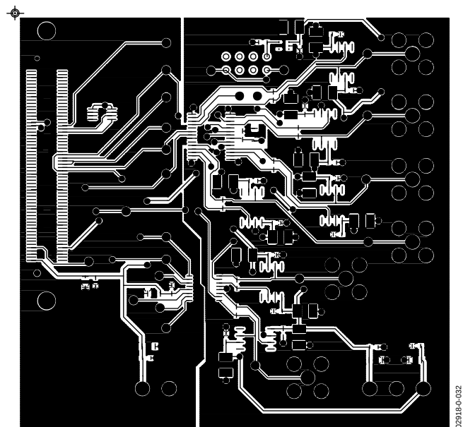
Figure 31. Component Side
