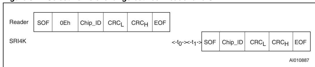
Figure 34. Select frame exchange between reader and SRI4K
