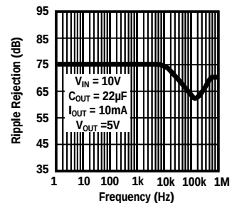
Ripple Rejection
