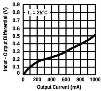
Dropout Voltage
