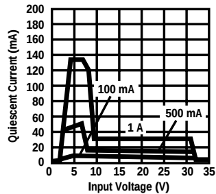
Quiescent Current
