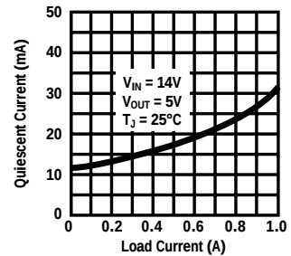
Quiescent Current
