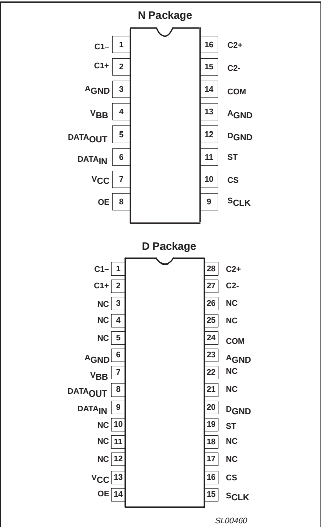
Figure 1. Pin configuration
