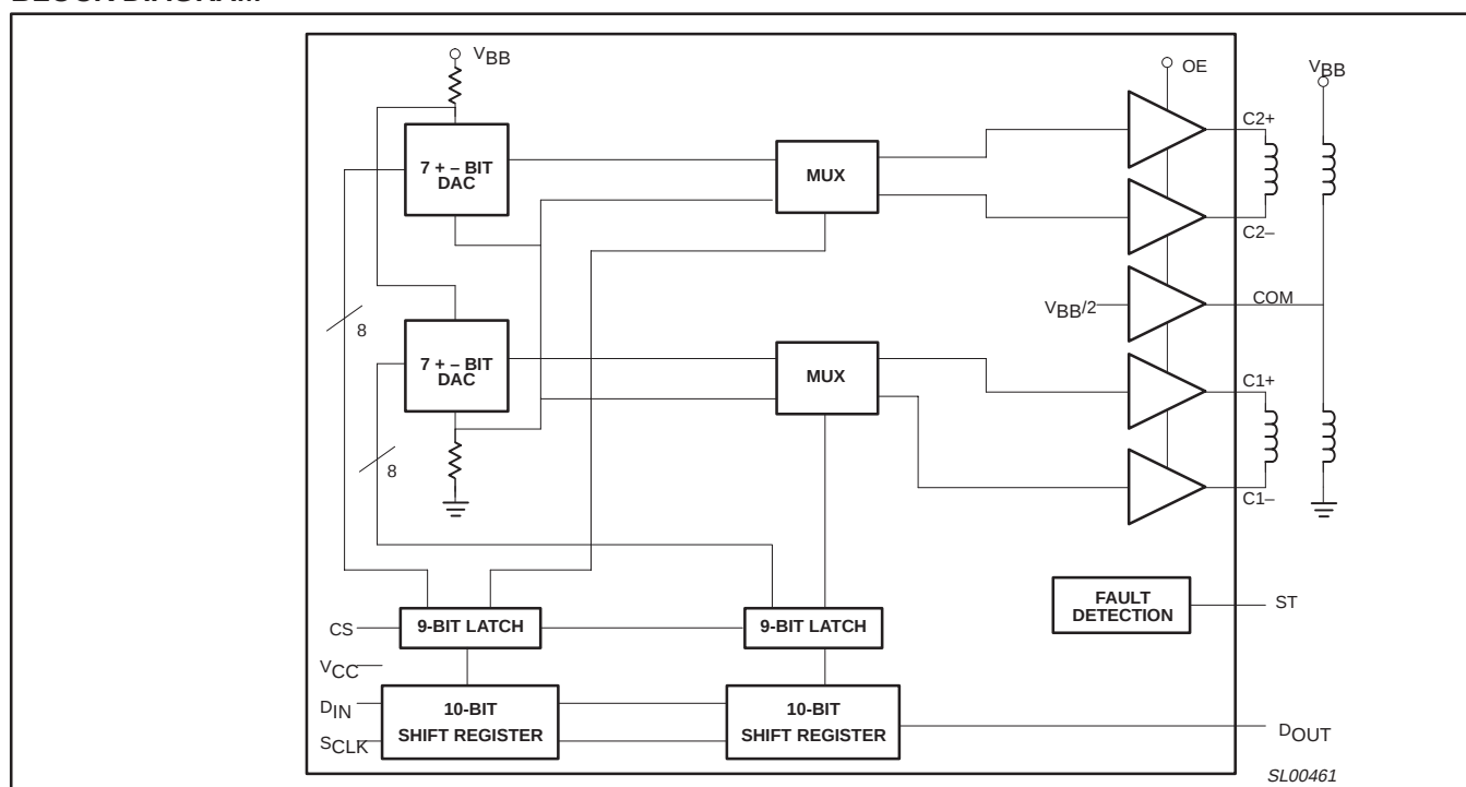
Figure 2. Block diagram
