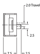
SS12SDH2LC Side Actuated
