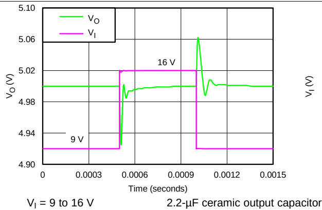
Figure 7. Input Voltage vs Output Voltage
