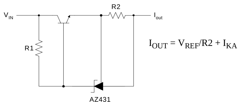
Figure19. Current Source or Current Limit
