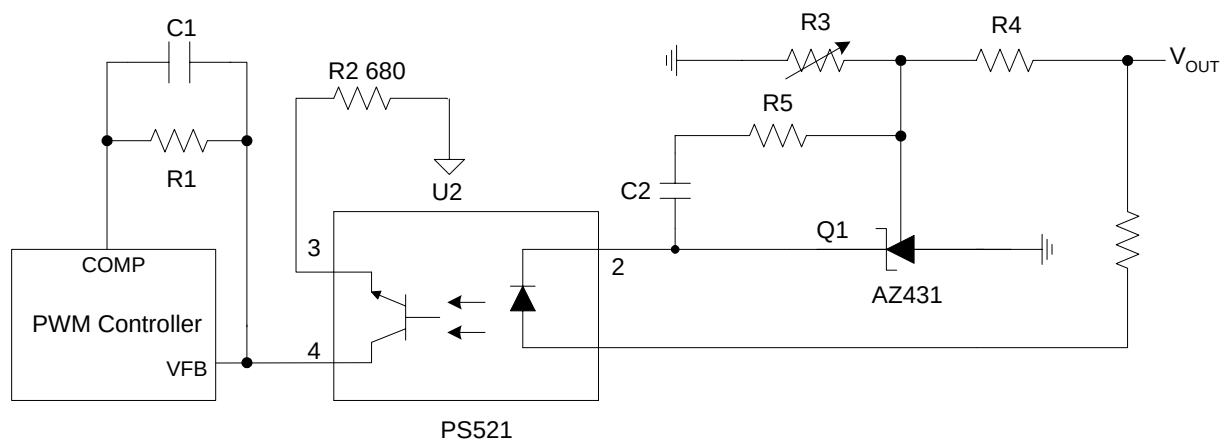
Figure 21. PWM Converter with Reference
