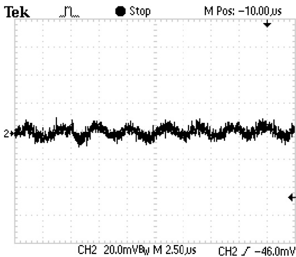
Output Noise (V IN =4.2V, I LOAD =100mA)
