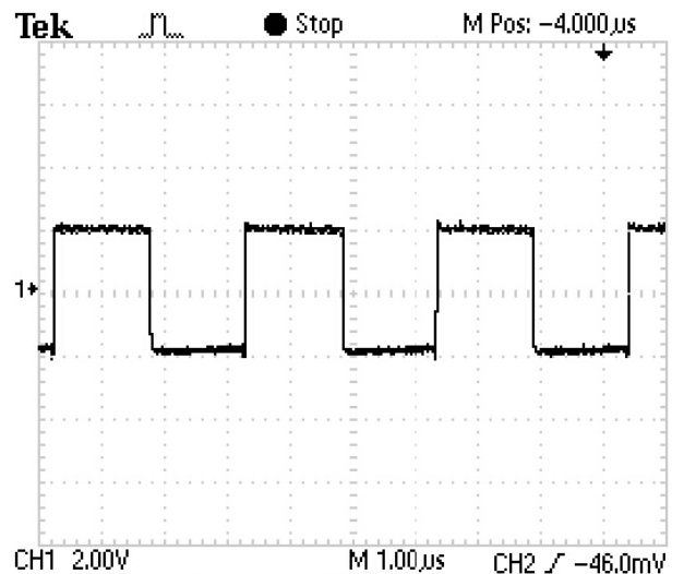
SW Noise (V IN =4.2V, I LOAD =100mA)
