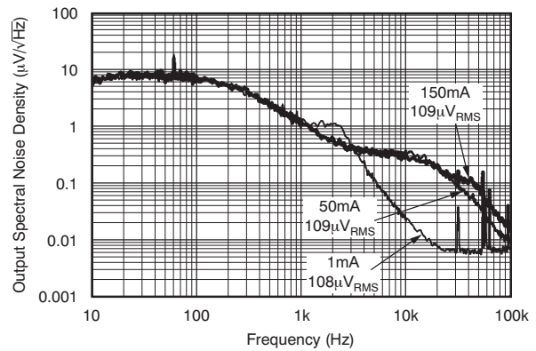
Figure 14. Output Spectral Noise Density vs Frequency, C_{IN} = 1\ \mu\text{F} , C_{OUT} = 2.2\ \mu\text{F} , V_{IN} = 3.2\text{ V} , TPS78227
