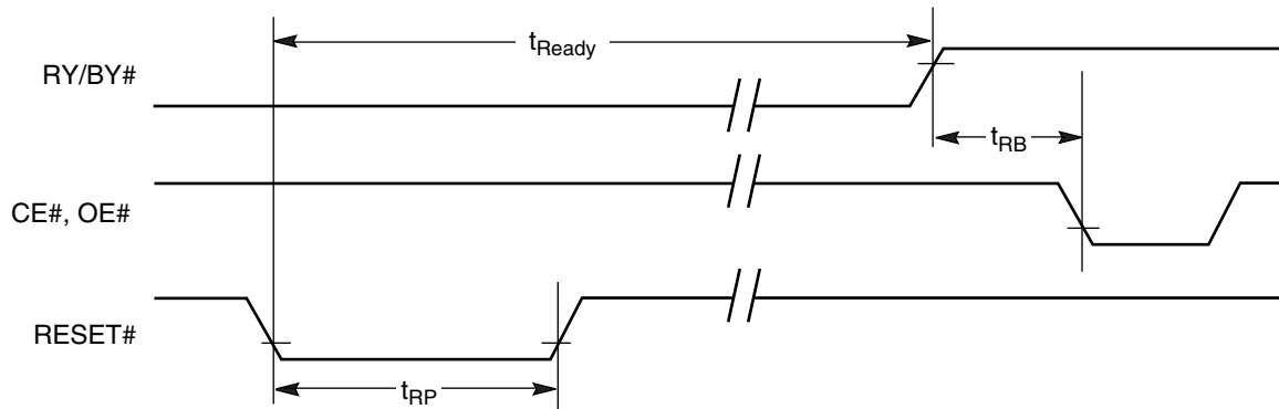
Reset Timings during Embedded Algorithms
