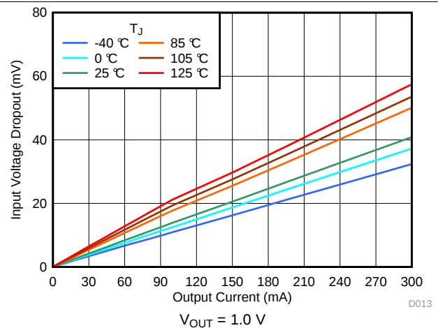
图 6. Dropout vs I_{OUT} and Temperature, YKA Package
