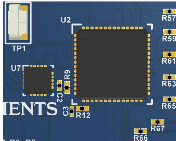
图 12-5. Example Layout (Top View in 3-D)
