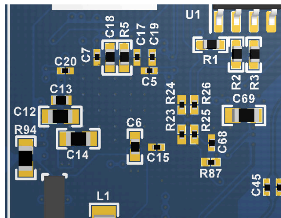
图 12-6. Example Layout (Bottom View in 3-D)
