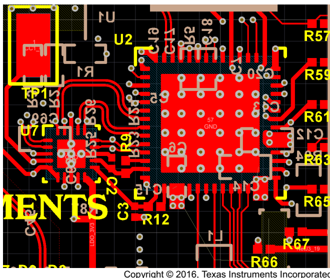
图 12-3. Example Layout (Top View in 2-D)
