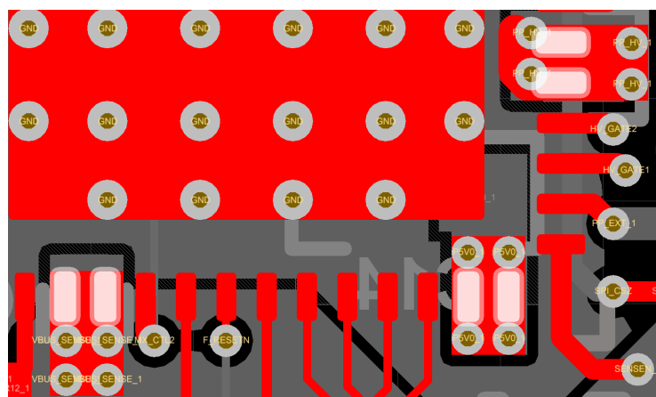
图 12-6. Example Layout (Bottom View in 3-D)
