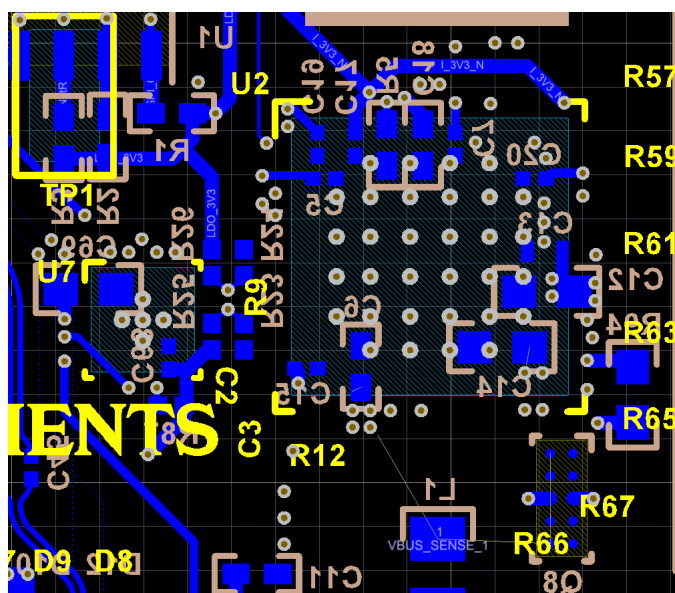
图 12-4. Example Layout (Bottom View in 2-D)
