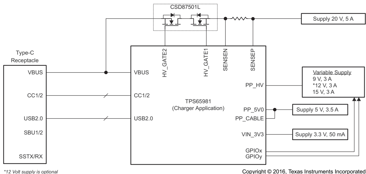
图 10-1. Type-C and PD Charger Application
