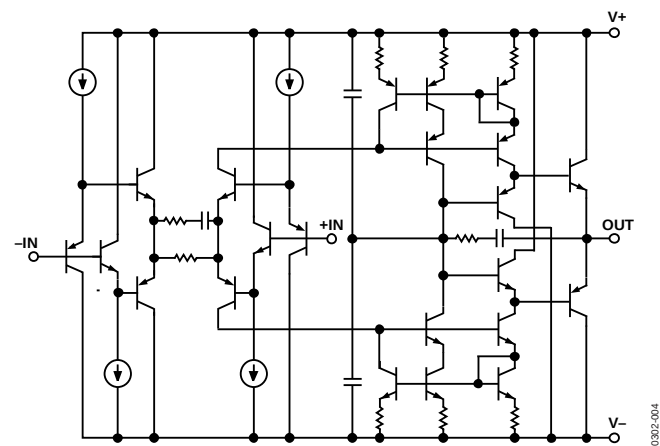
Figure 4. Simplified Schematic
