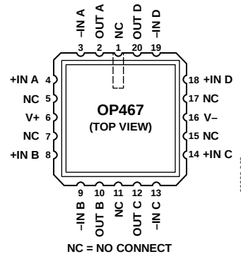
Figure 3. 20-Terminal LCC (RC Suffix)
