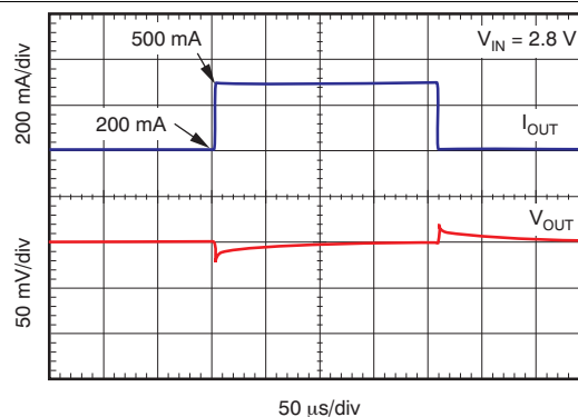
Figure 14. Load Transient Response 200 mA to 500 mA, C_{OUT} = 10\text{ }\mu\text{F}
