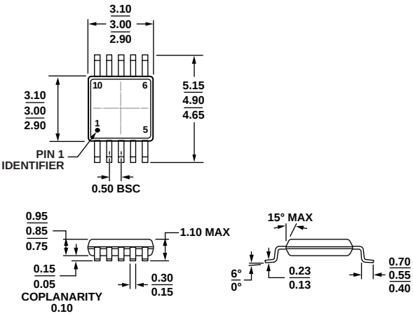
COMPLIANT TO JEDEC STANDARDS MO-187-BA Figure 27. 10-Lead Mini Small Outline Package [MSOP] (RM-10) Dimensions shown in millimeters
