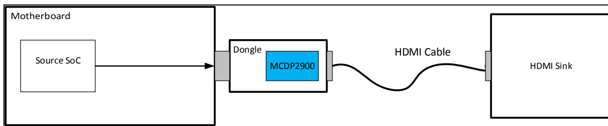
Figure 2. MCDP2900 adaptor (dongle) use case
