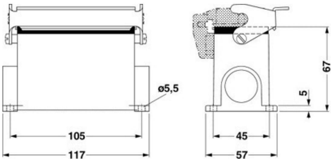
Dimensioned drawing
