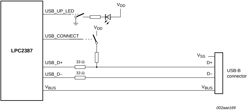
Fig 13. LPC2387 USB device port configuration
