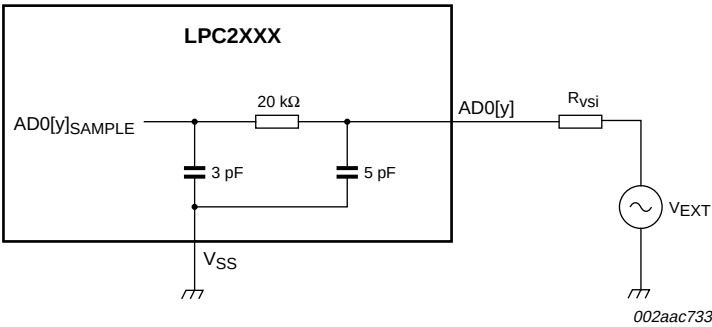
Fig 5. Suggested ADC interface - LPC2387 AD0[y] pin
