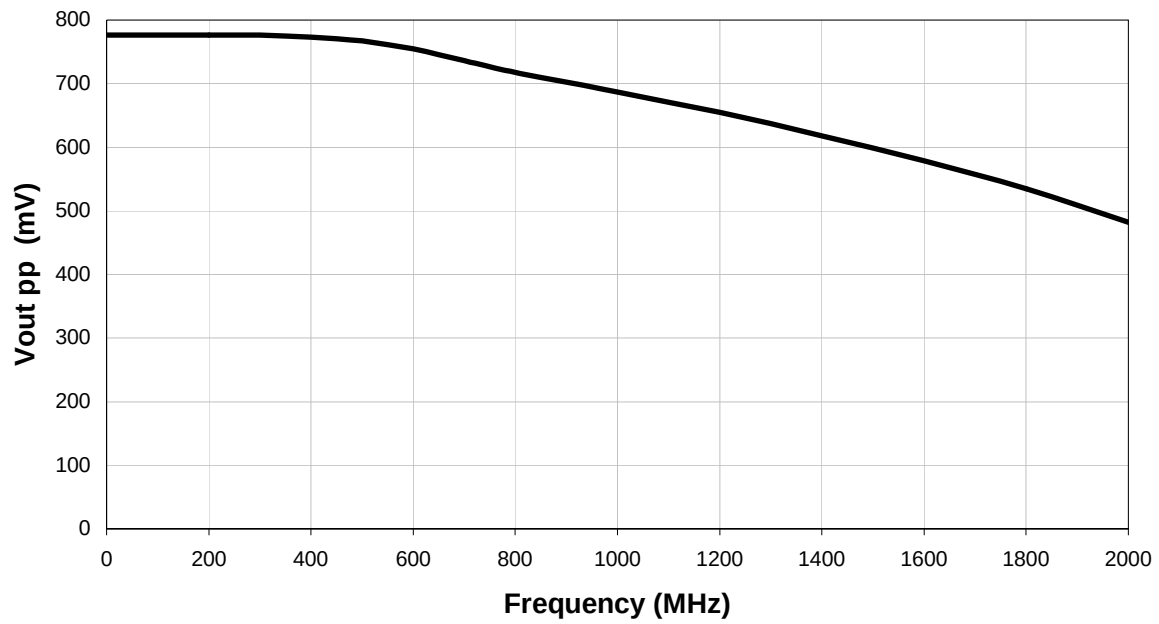
Fig. 1 Typical Output Swing Versus Frequency for AZ100LVEL11
