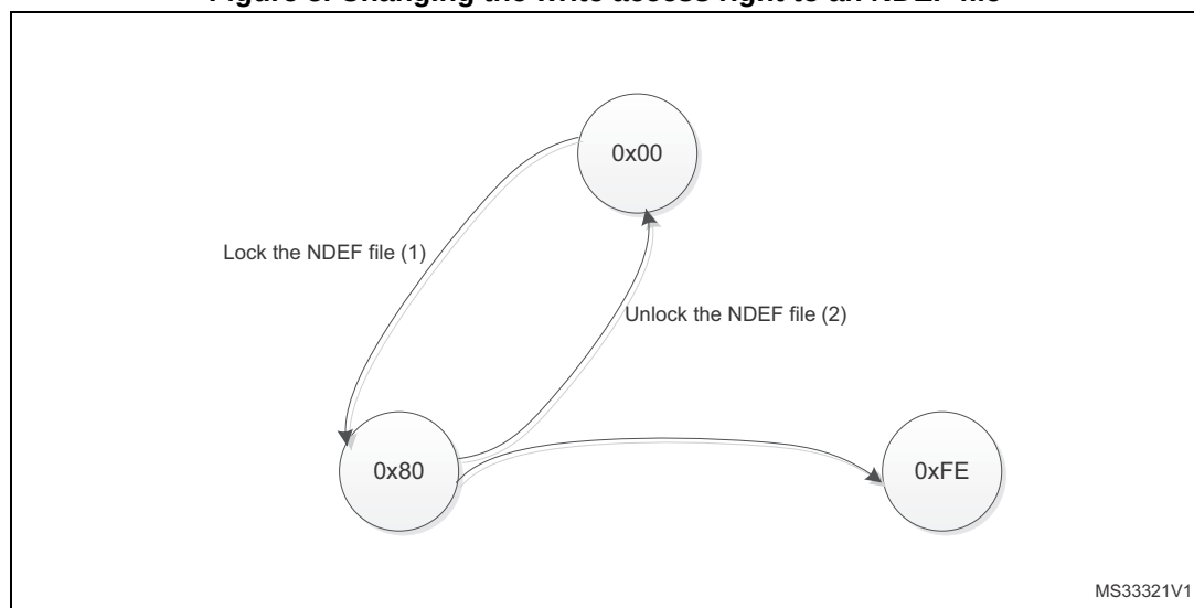
Figure 5. Changing the write access right to an NDEF file
