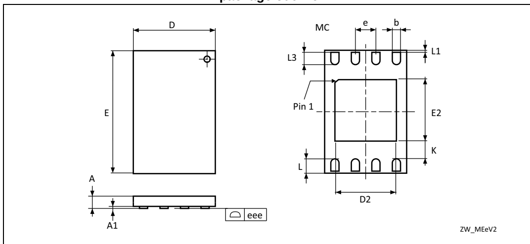
Figure 6. UFDFPN8 - 8-lead ultra thin fine pitch dual flat package, no lead, 2x3 mm, package outline
