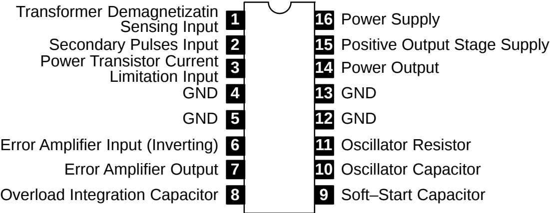
Pin Connection Diagram
