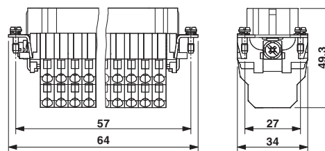
Female contact insert
