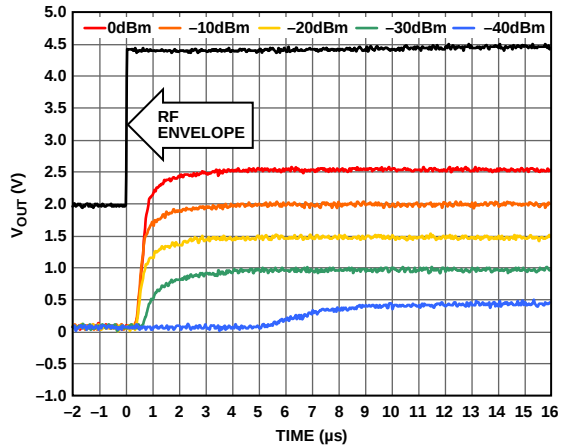
Figure 21. Output Response to RF Burst Input, Carrier Frequency at 2.14 GHz, C_{LPF} = 390 pF, C_{HPF} = \text{Open} , Rising Edge
