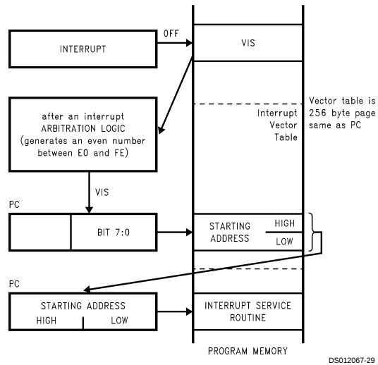
FIGURE 36. VIS Operation
