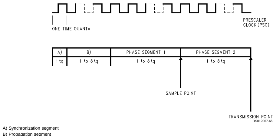
FIGURE 31. Bit Timing
