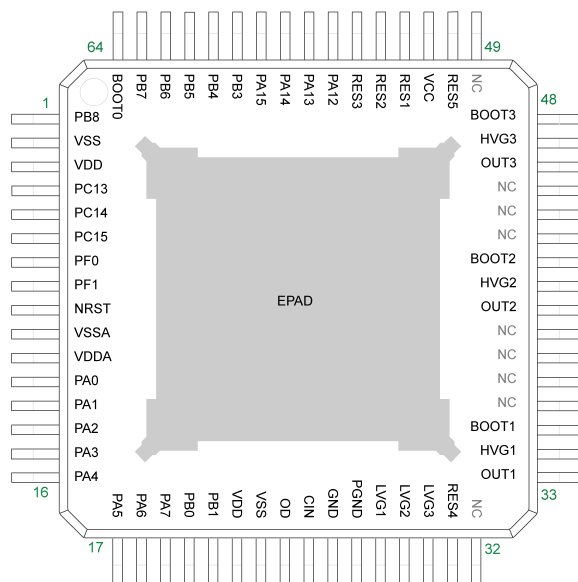
Figure 2. STSPIN32F025x pin connection (TQFP top view)
