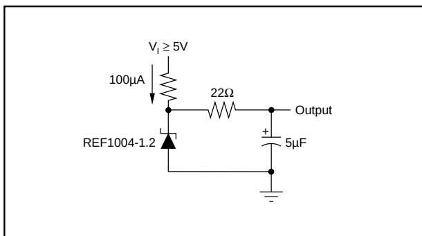
FIGURE 1. Low-Noise Reference.
