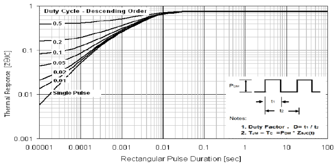
Transient Thermal Response Curve For JCS4N65RE/VE/BE/ME/MFE
