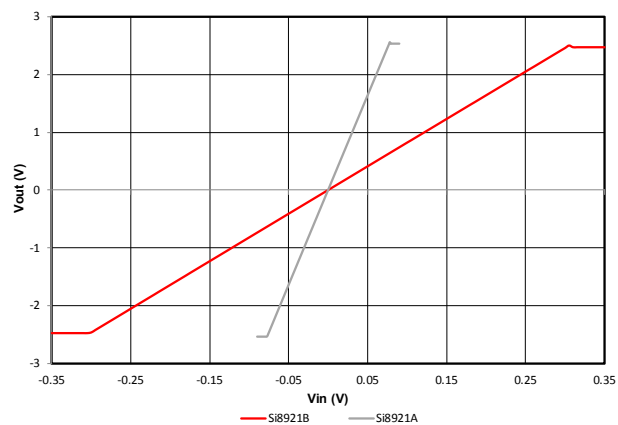
Figure 4.15. Si8921 Output Voltage (V) vs. Input Voltage (V)
