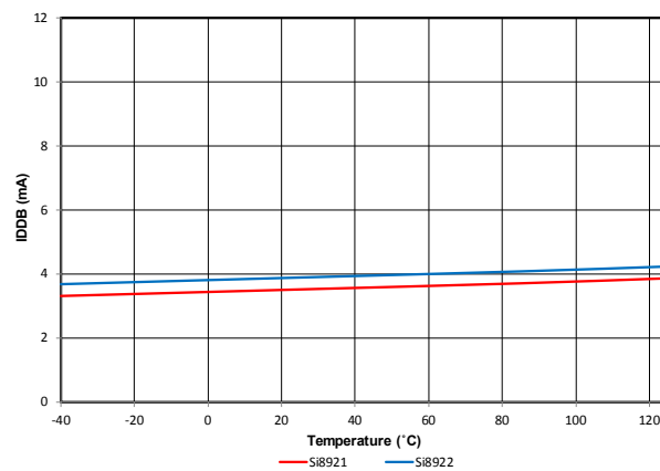
Figure 4.29. IDDB (mA) vs. Temperature (°C)
