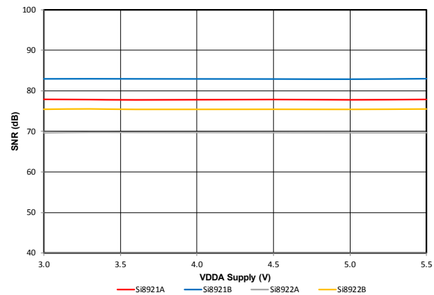
Figure 4.11. Signal-to-Noise Ratio (dB) vs. VDDA Supply (V)
