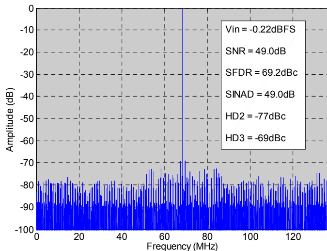
Figure 14. Output Spectrum at 68.465MHz
