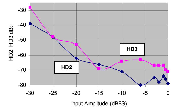
Figure 5. HD2, 3 vs. Vin
