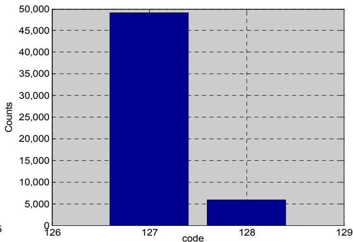
Figure 12. Noise Histogram
