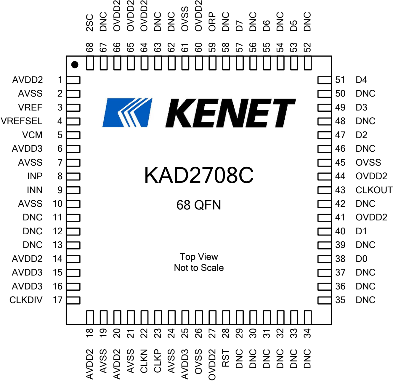
Figure 2. Pin Configuration
