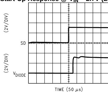
Start-Up Response @ V_{IN} = 2.7\text{V} (LM2794)
