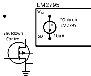
Figure 2. Open-Drain Logic Shutdown Control
