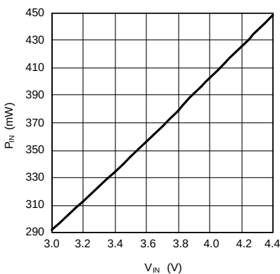
Figure 8. P_{IN} vs V_{IN} 4 LEDs, 2.5 \leq V_{DX} \leq 3.9V , I_{DX} = 15mA
