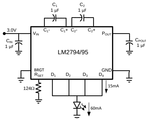
Figure 6. One Parallel Connected LED
