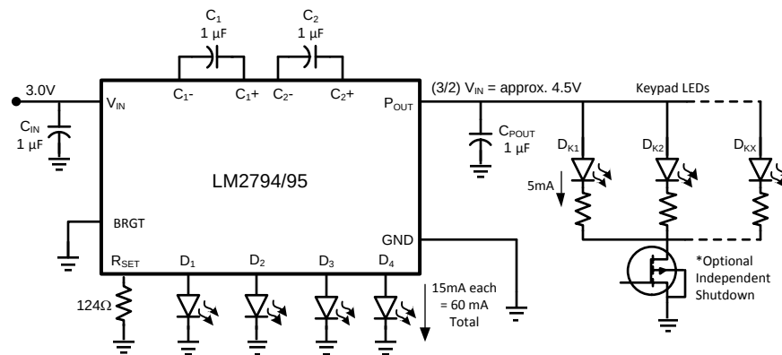
Figure 3. Keypad LEDs Connected to P OUT
