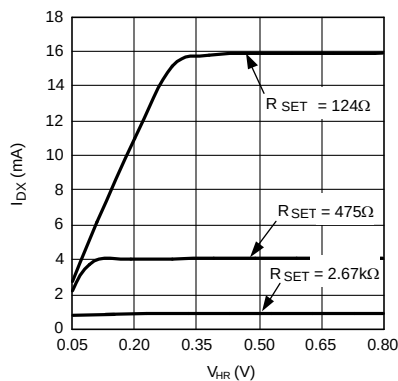
Figure 4. I_{LED} vs V_{HR} 4 LEDs, V_{IN} = 3.0V
