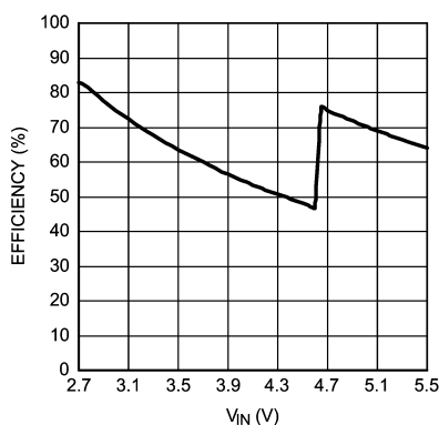
Figure 7. Efficiency vs V_{IN} 4 LEDs, V_{LED} = 3.6V , I_{LED} = 15mA
