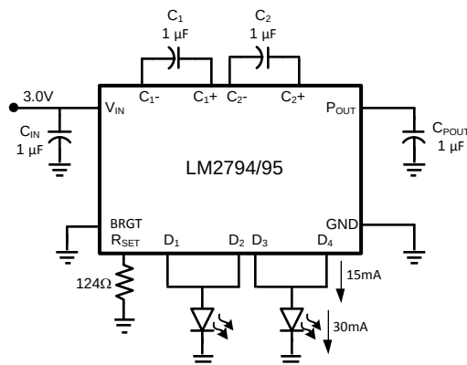
Figure 5. Two Parallel Connected LEDs
