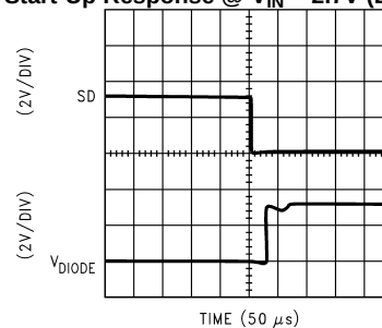
Start-Up Response @ V_{IN} = 2.7\text{V} (LM2795)
