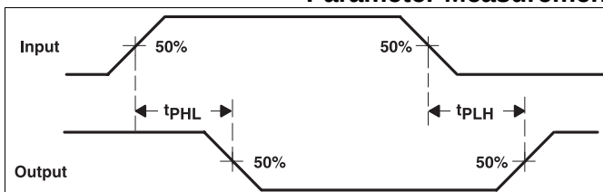
VOLTAGE WAVEFORMS
