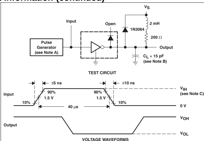
VOLTAGE WAVEFORMS
