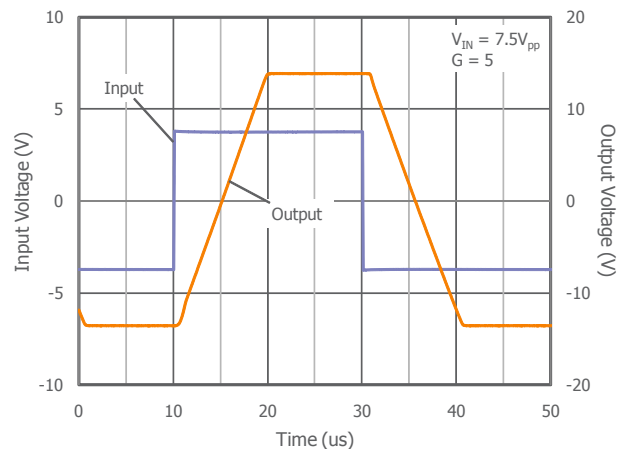
Figure 6. Overdrive Recovery
