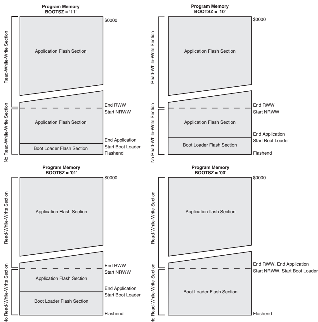
Figure 24-2. Memory Sections (1)
