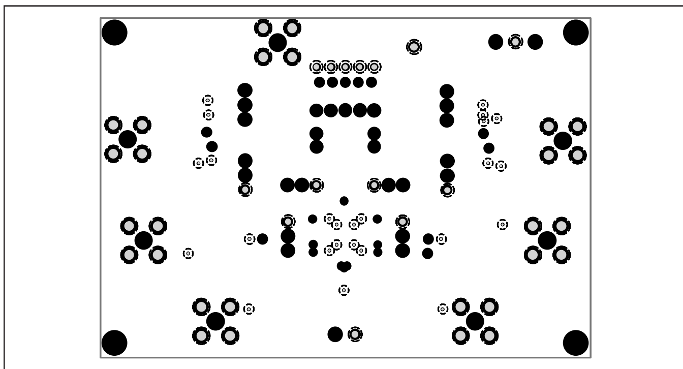
FIGURE 3. Ground Layer.
