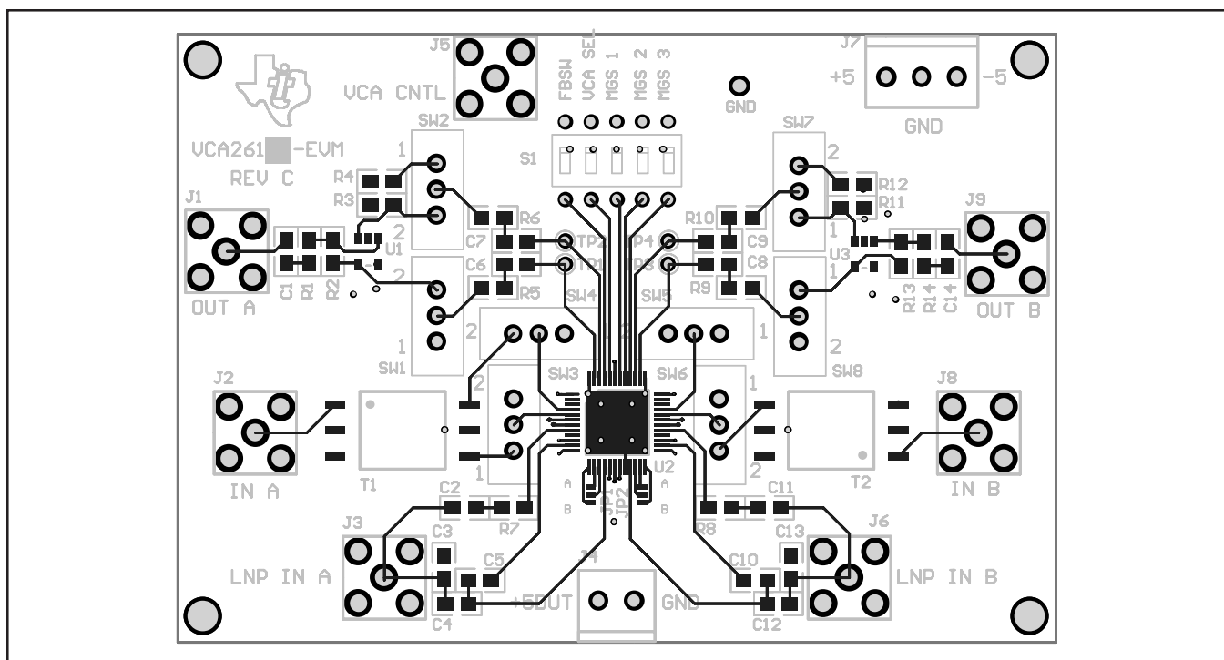
FIGURE 2. Top Layer and Silkscreen.
