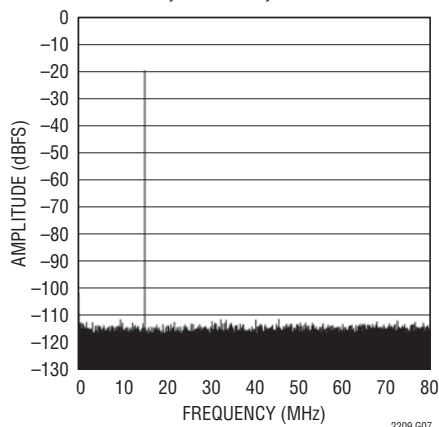
64k Point FFT, f_{IN} = 15.1\text{MHz} , -20dBFS, PGA = 0, Dither "On"
