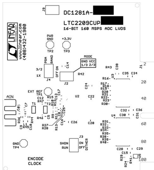
Silkscreen Top
