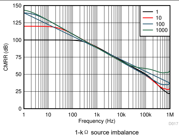
图 7-18. CMRR vs Frequency (RTI)
