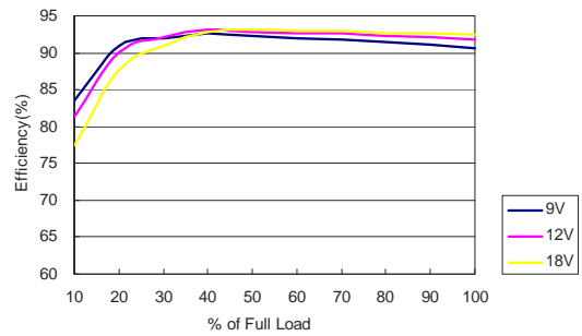
MKW50-12S12 Efficiency vs Load Current
