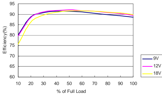
MKW50-12S033 Efficiency vs Load Current
