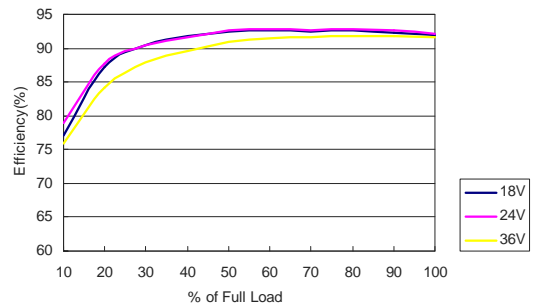
MKW50-12S24 Efficiency vs Load Current
