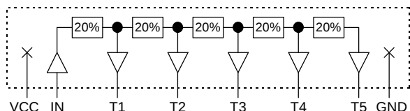
Functional diagram for dash numbers >= 25
