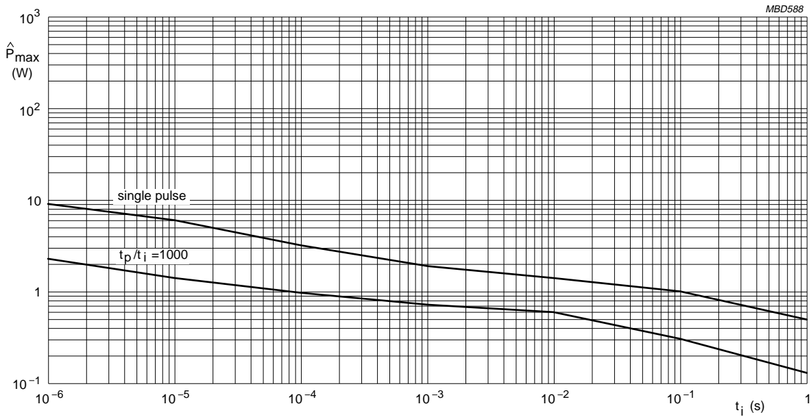
Fig.7 Pulse on a regular basis for type: RC11 ; maximum permissible peak pulse power ( \hat{P}_{max} ) as a function of pulse duration for R \leq 10 \text{ k}\Omega , single pulse and repetitive pulse t_p/t_i = 1000 .
