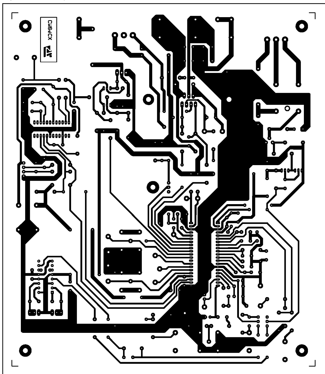
Figure 24 : PCB Layout
