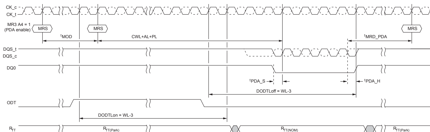
Figure 61: PDA Operation Enabled, BL8
