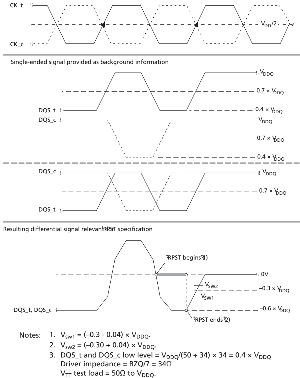
Figure 128: t_{RPST} Method for Calculating Transitions and Endpoints
