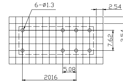
BOTTOM VIEW (1B)
