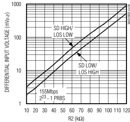
POWER-DETECT THRESHOLD vs. R2 ( R_1 = 100k\Omega )
