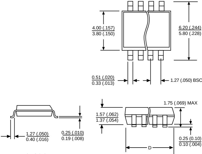
Surface Mount Narrow Body (D); 150 mil wide
