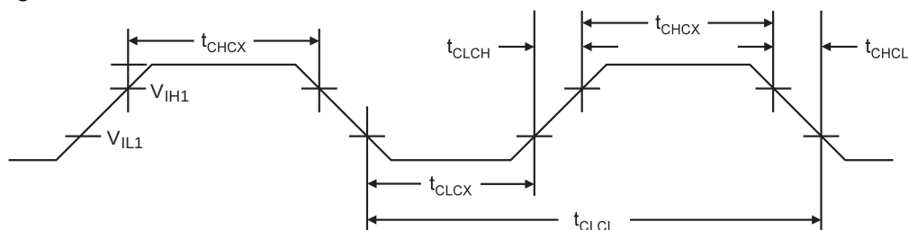
Figure 81. External Clock Drive Waveforms
