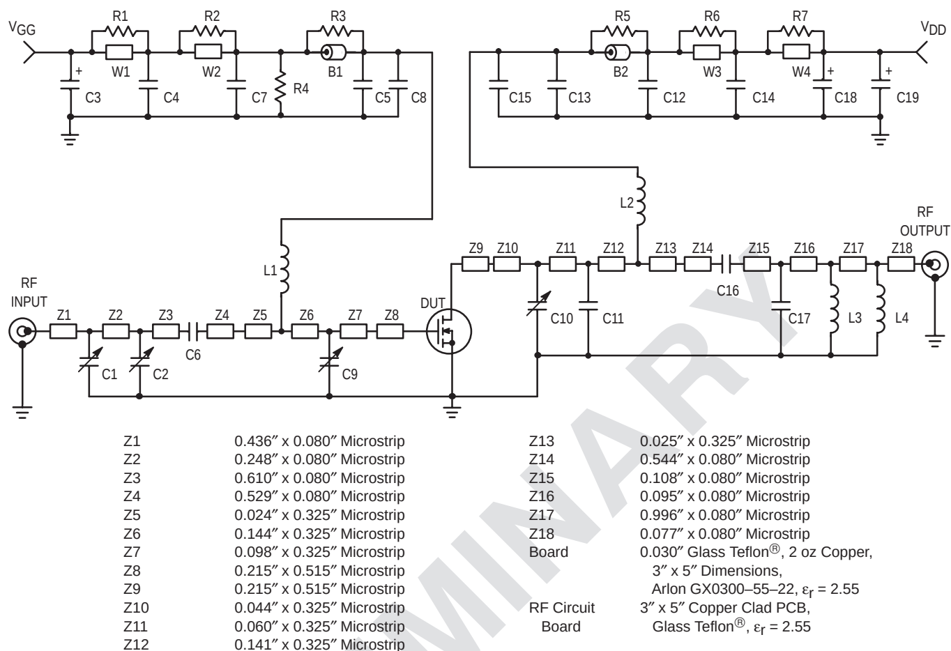
Figure 1.193 – 2.0 GHz Broadband Test Circuit Schematic
