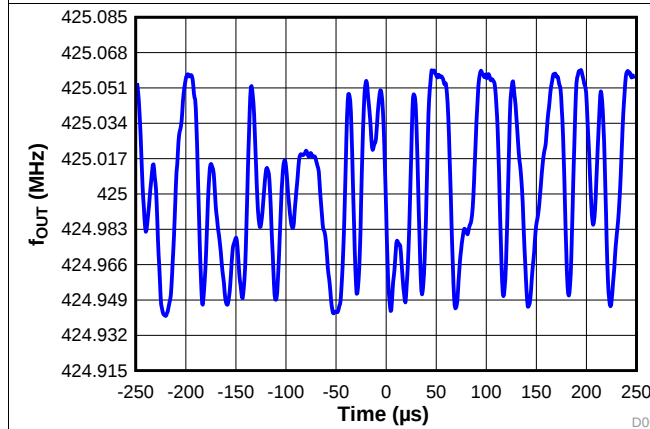
图 29. 4-Level GFSK Modulation
