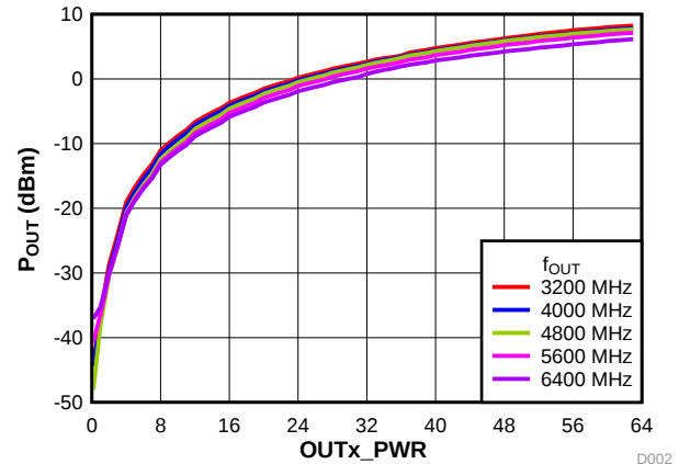
图 166. Output Power vs Power Control Bits
