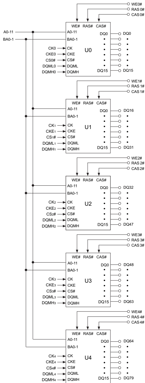
FIGURE 2 – FUNCTIONAL BLOCK DIAGRAM
