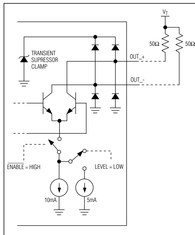
Figure 3. Simplified Output Circuit Without Back Termination Resistor
