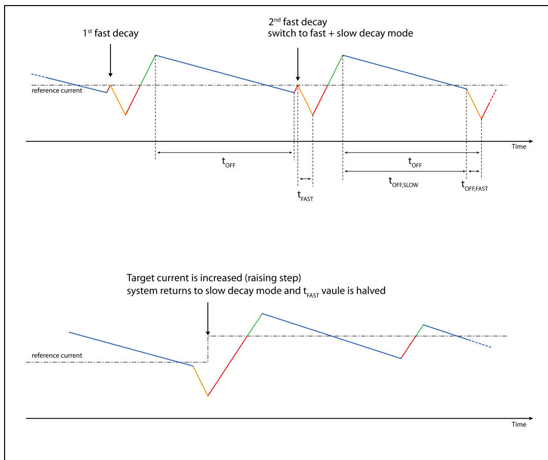
Figure 18. Adaptive decay switch from normal to slow+fast decay mode and viceversa
