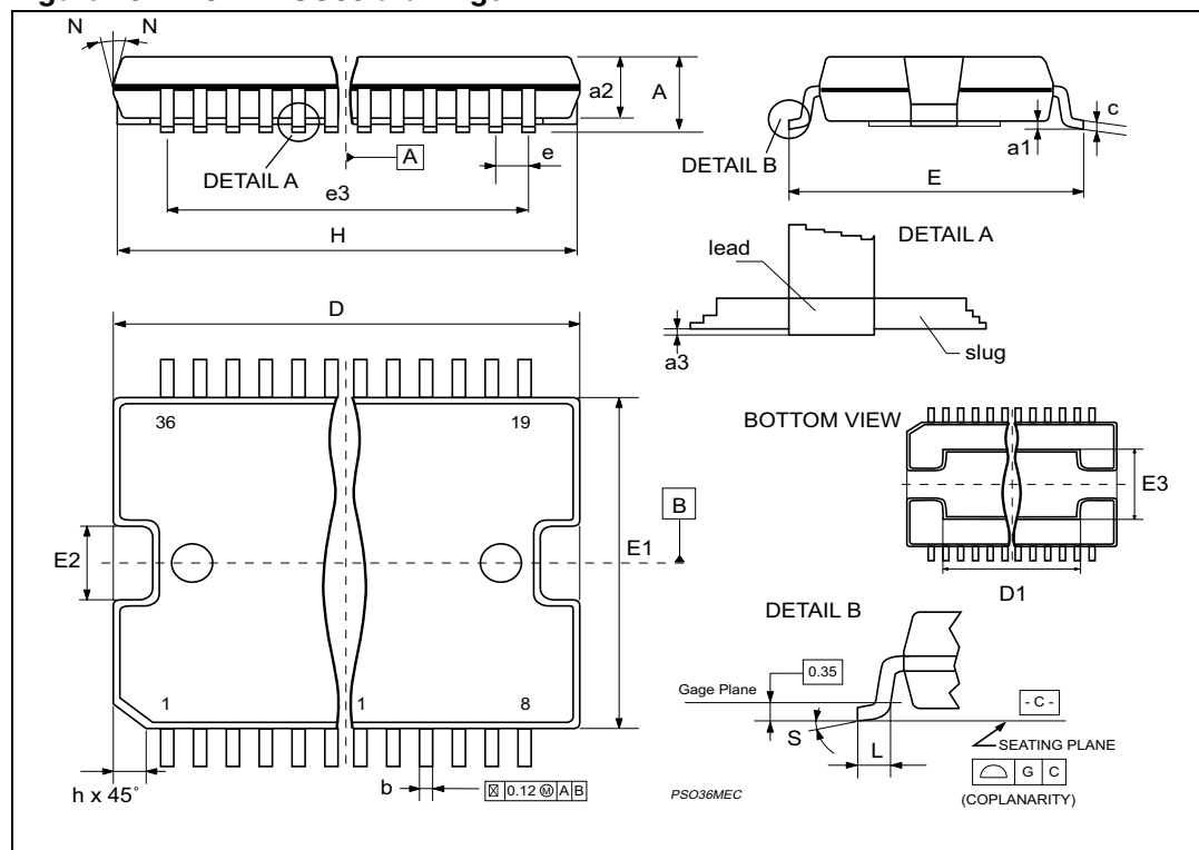
Figure 26. POWERSO36 drawings
